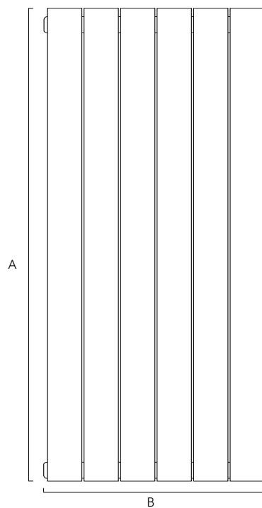
OSCA10X6 - 1046mm x 500mm
