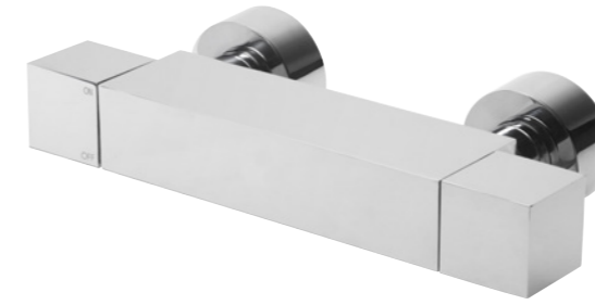
Factor bottom outlet bar valve - single function 265(w) x 40 x 106mm(d) Minimum pressure 0.1bar
