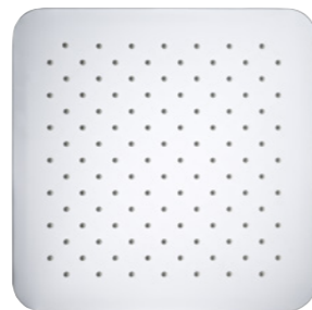
Square 300mm ceiling flush mounted stainless steel overhead shower 300(w) x 300mm(d) Minimum pressure 1.0bar
