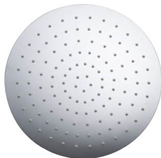
Round 300mm ceiling flush mounted stainless steel overhead shower 300mm(dia) Minimum pressure 1.0bar
